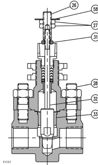
Figure 3. NPS 1/2 (12.7 mm) Integral Seating for Cv = 1.0, 1.5, and 2.5 Class IV Shutoff
