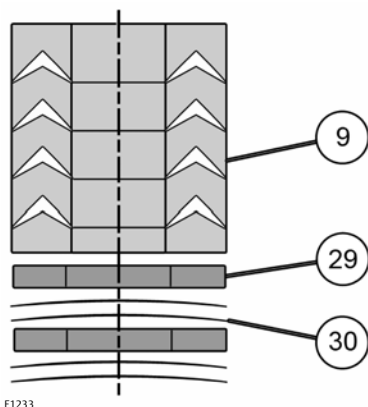
Figure 4. V-Ring Packing Kit
