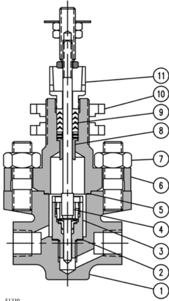
Figure 1. NPS 1/4 and 1/2 (6.35 and 12.7 mm) Soft Seat Cage Design for Cv = 0.00013 to 0.45 Class VI Shutoff (N10276 Nickel Alloy Construction Available)
