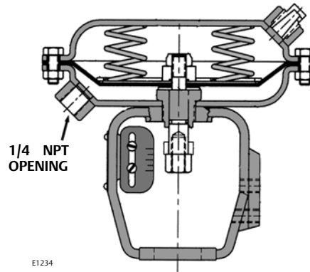
Figure 5. Baumann 16 Actuator Sectional
