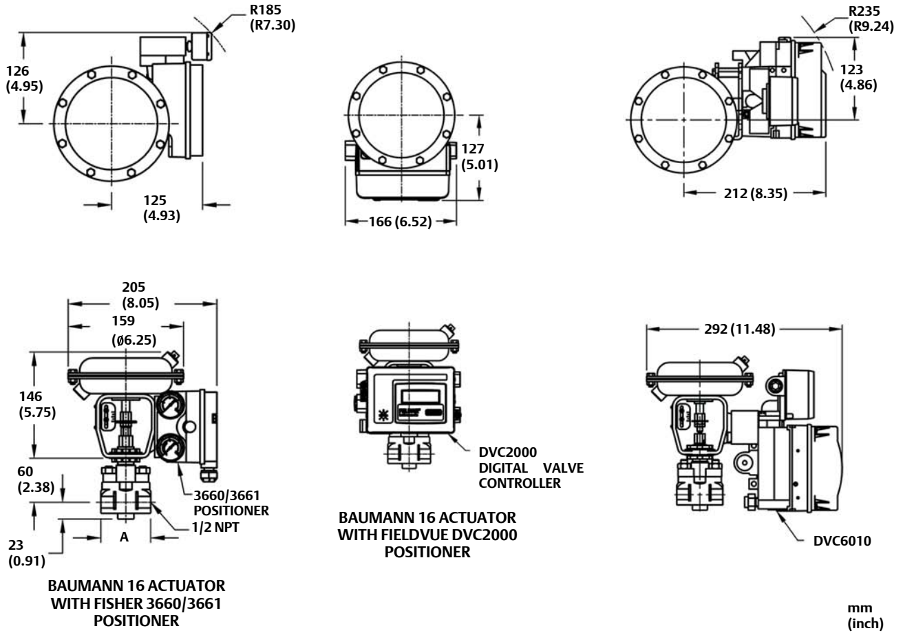
Figure 9. Dimensional Drawings
