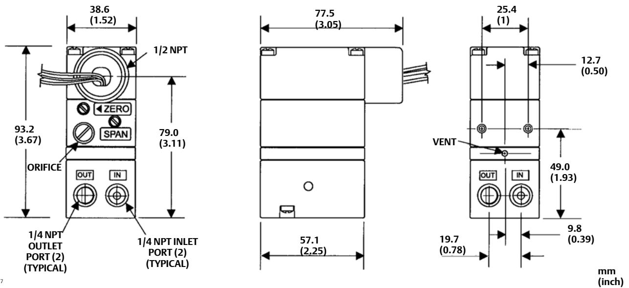
Figure 8. TA6000 Electropneumatic Transducer Dimensions
