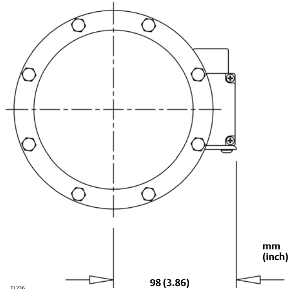
Figure 7. Baumann 16 Actuator with TA6000 (Top View)
