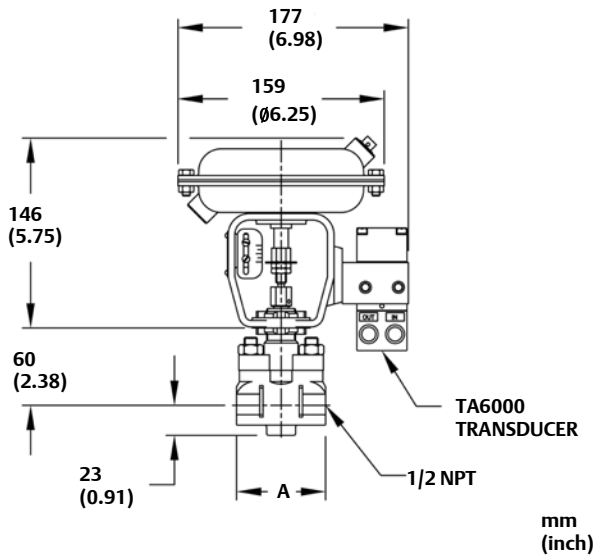
Figure 6. Baumann 16 Actuator (Front View)
